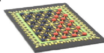
Figure 2 Zamma gameboard
